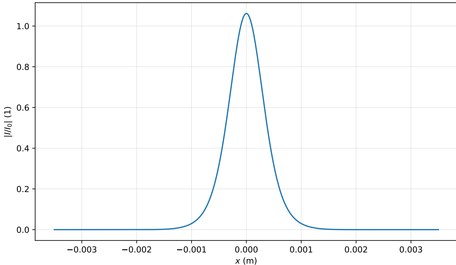
Intensity profile I(x, y = 0, z = 1.513m)/I_0 , P_{in}=0.6P_{cr} , artificial time
